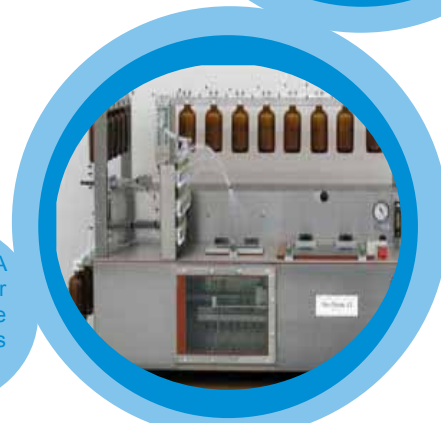
MerMade 6/12 DNA Synthesizer For medium scale oligonucleotide synthesis
